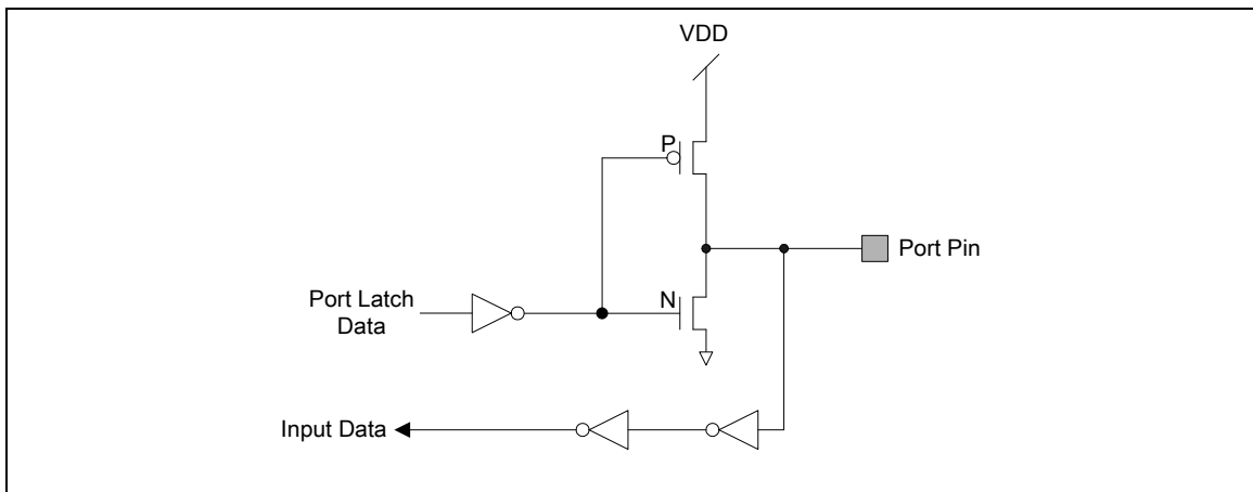
Figure 6-11 Push-Pull Output
